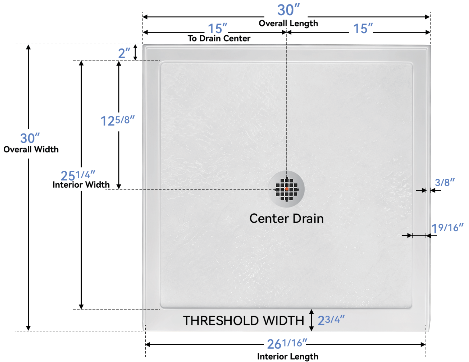
Top View
