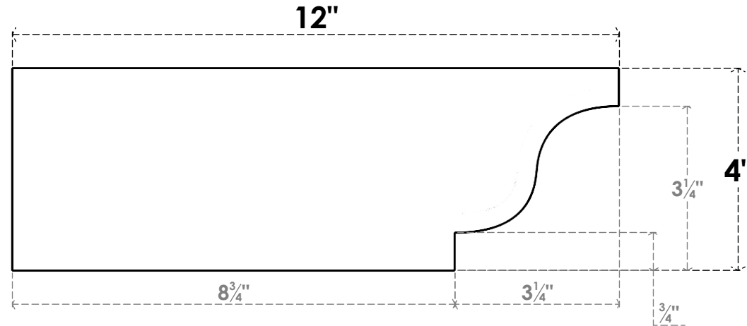
SIDE PROFILE
