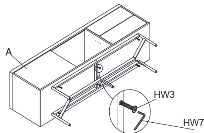
STEP2 assemble the metal base with the body
