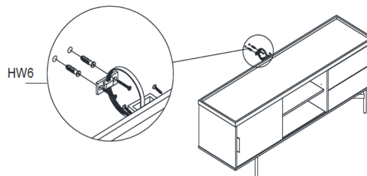
STEP2 assemble the metal base with the body
