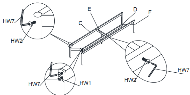
STEP1 assemble the metal base
