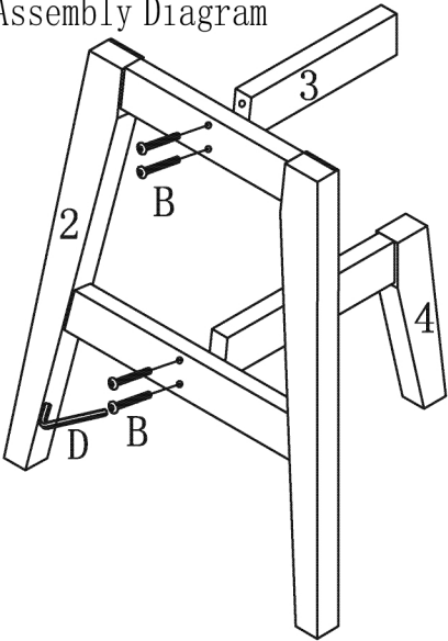
Layer Board Assembly Drawing
