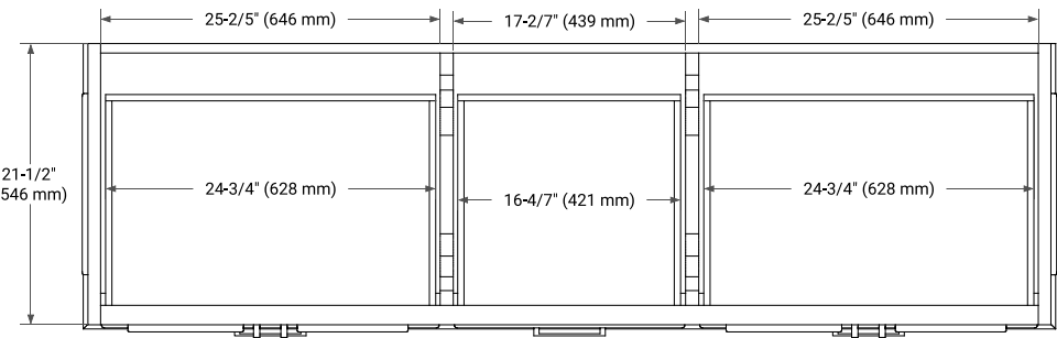
PLAN VIEW
