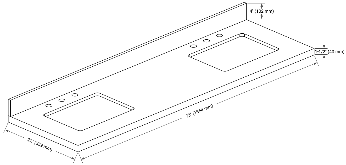
THREE DIMENSIONAL COUNTERTOP VIEW
