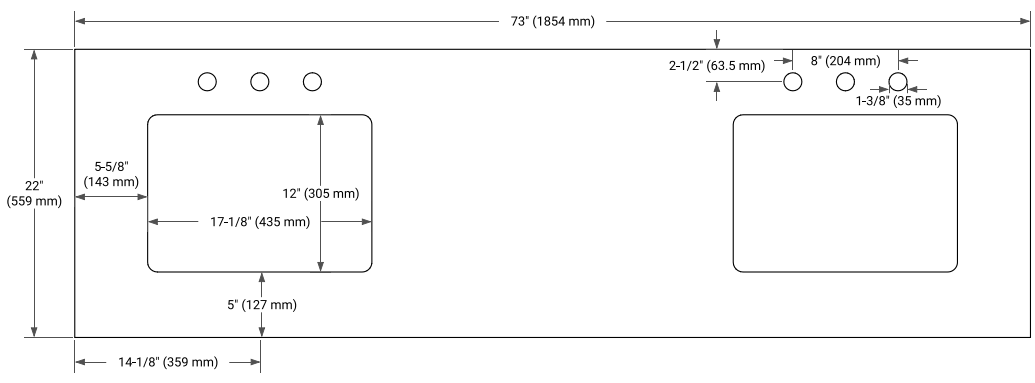
COUNTERTOP PLAN VIEW
