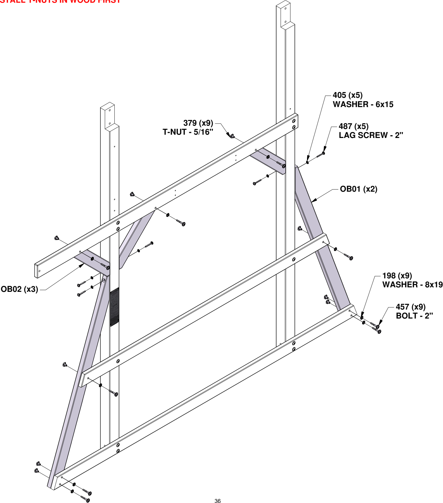
OB02 DECK BRACE - W4L21070 (x3) 1 1/8"x2 7/8"x17" (30x72x433)
