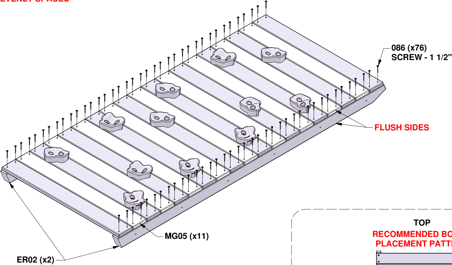
RIGHT ROCK ASSEMBLY (x2)
