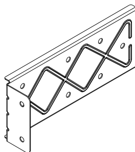
A4M05882 EXTENDED SWING BEAM BRACKET (x2)
