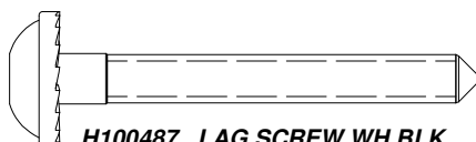
H100487 LAG SCREW WH BLK (x12) 1/4x2
