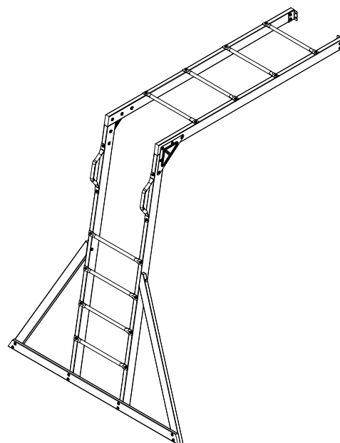
9250352 MONKEY BAR ASSEMBLY (x1)
