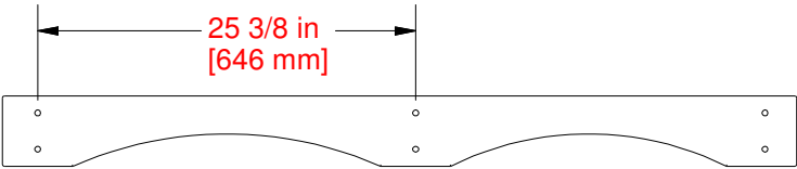
HT01 WALL RAIL - W4L21095 (x1) 1"x4 3/4"x53 3/8" (24x120x1357)
