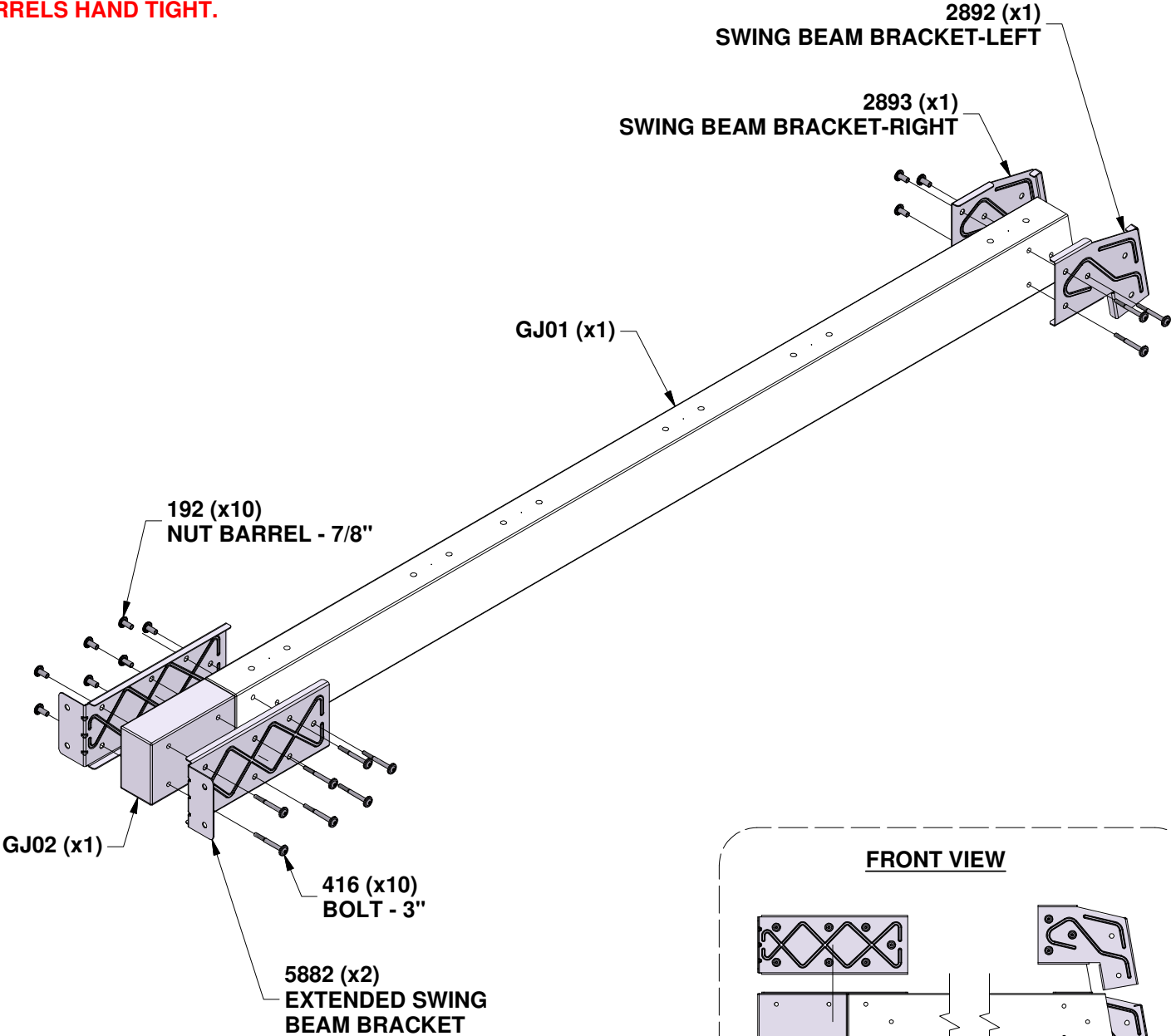
A4M05882 EXTENDED SWING BEAM BRACKET (x2)
