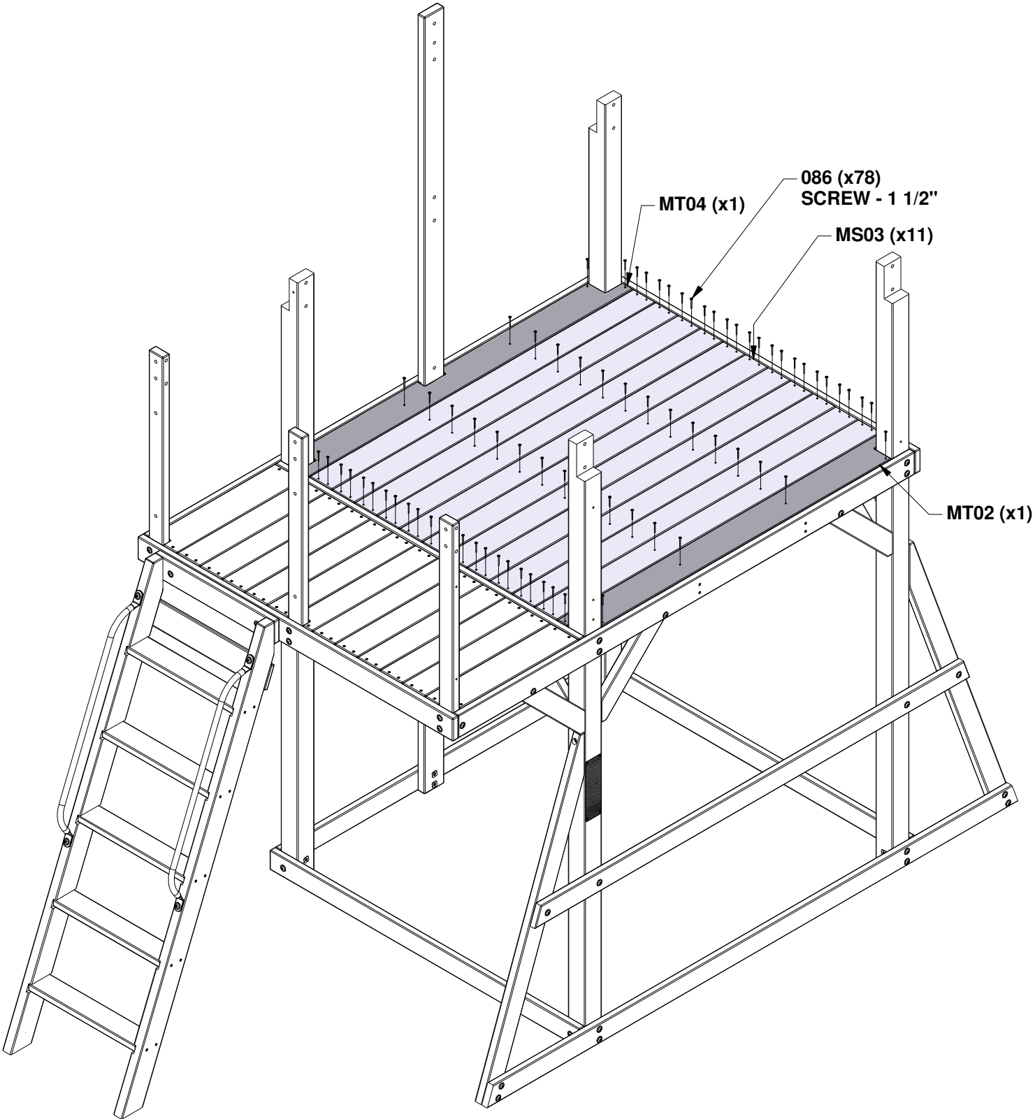
MT04 FLOOR BOARD - W4L21118 (x1) 5/8"x4 3/4"x54 5/8" (16x120x1389)
