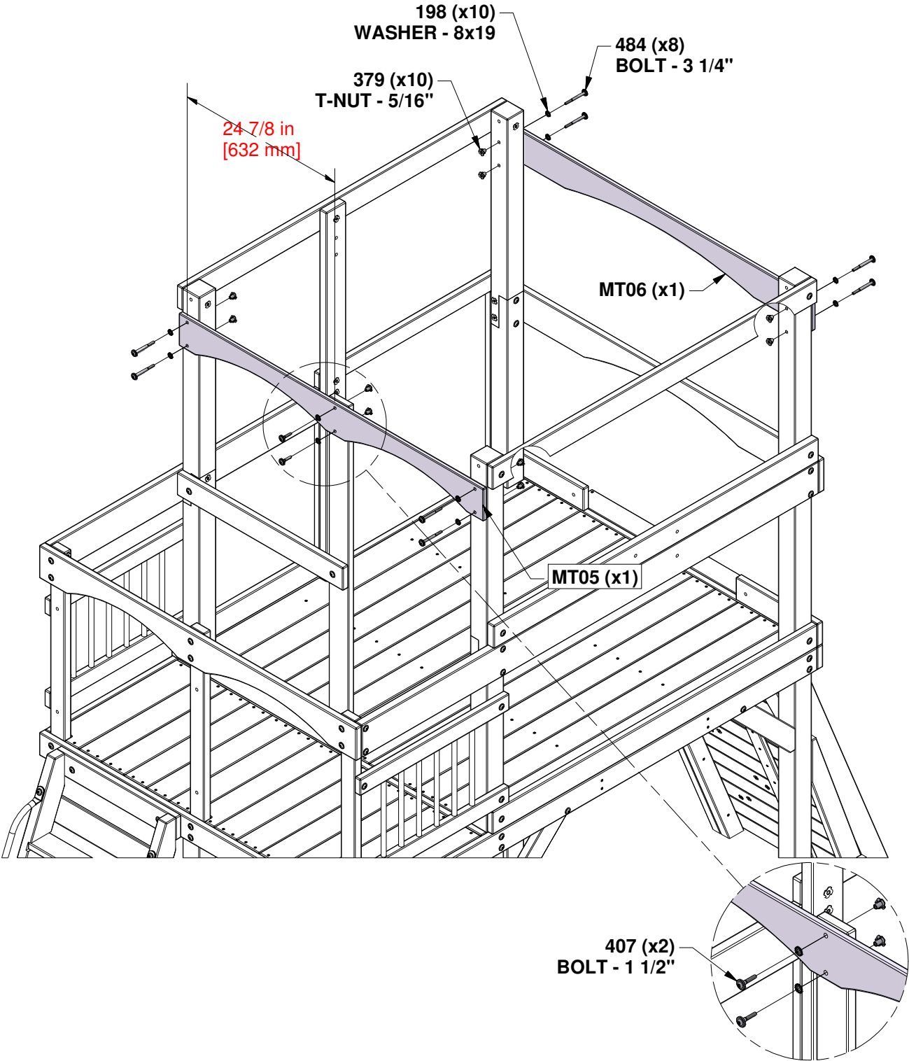
MT05 WALL RAIL - W4L21113 (x1) 5/8"x4 3/4"x51 1/4" (16x120x1303)
