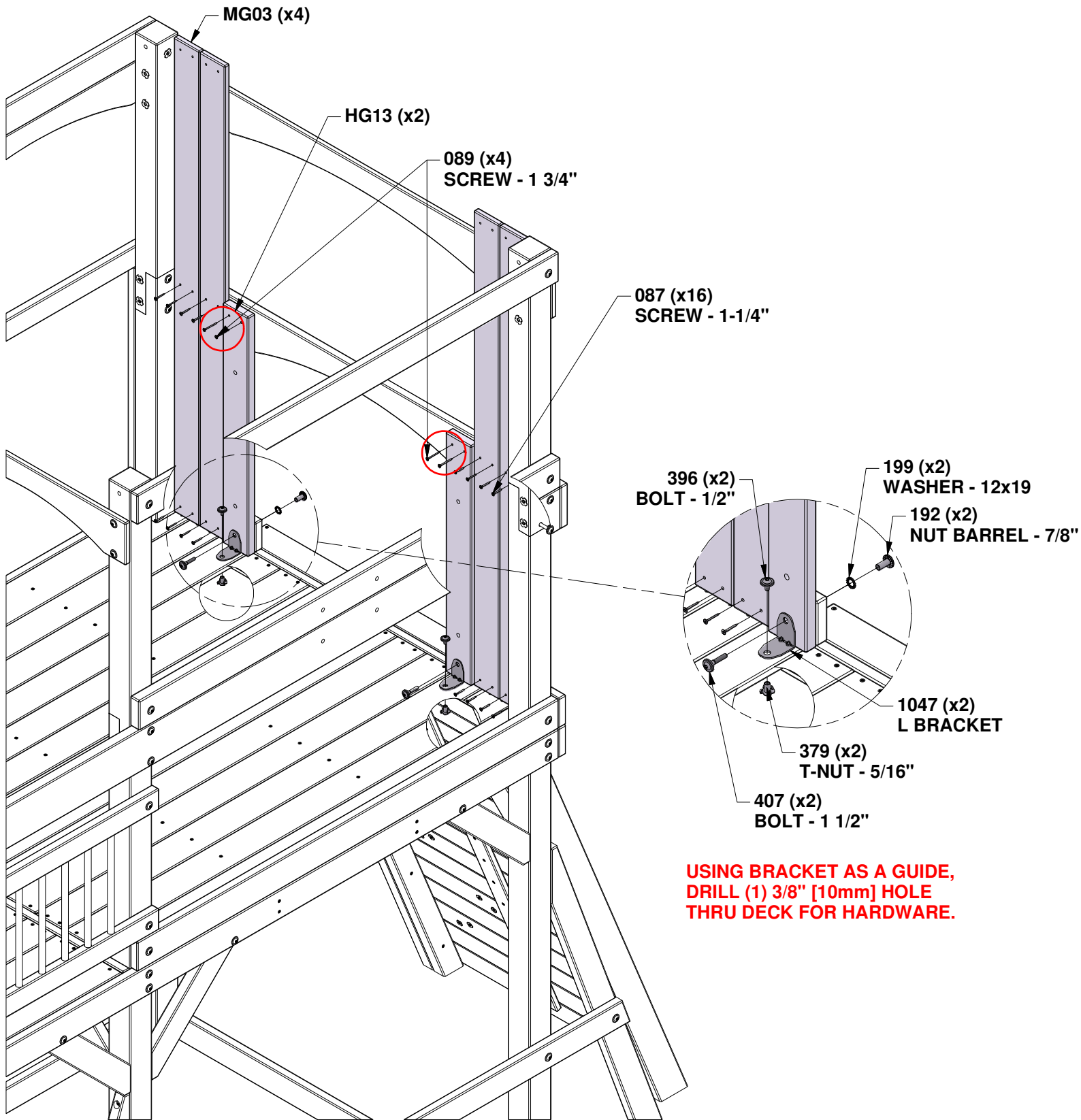
MG03 WALL BOARD - W4L21135 (x4) 5/8"x3 1/4"x53 1/4" (16x84x1354)
