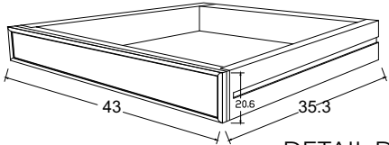
DETAIL DRAWER
