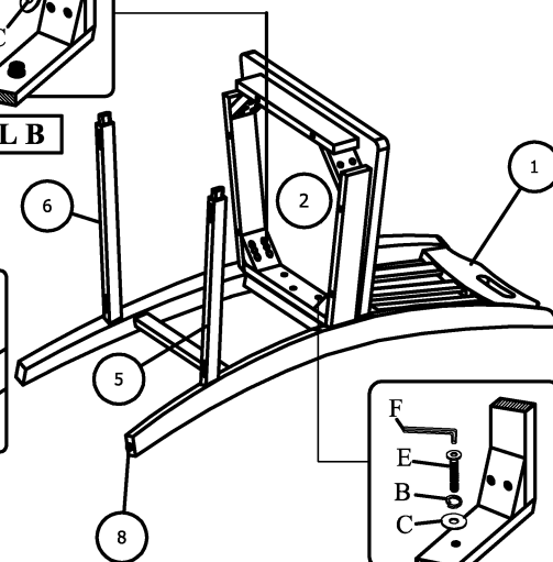
DETAIL A
