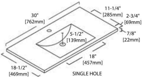
SINGLE HOLE
