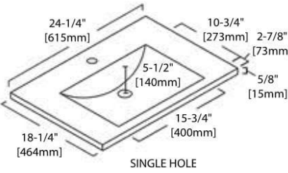
SINGLE HOLE
