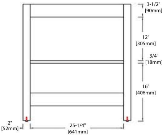
BACK VIEW
