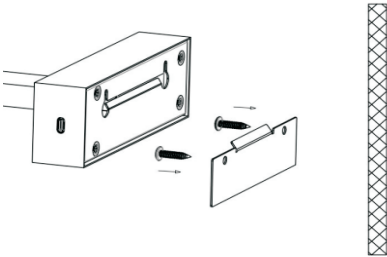
A. Installation with screws mounting
