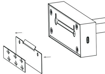
B. Or installation with 3M sticking
