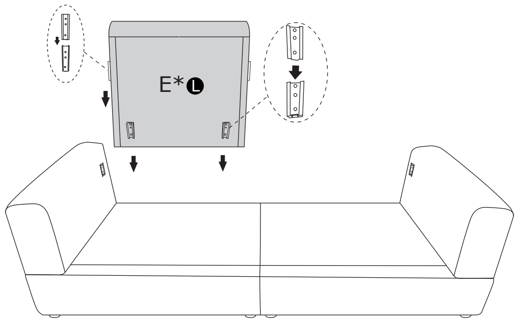
DIAGRAM 5 :Assembled back
