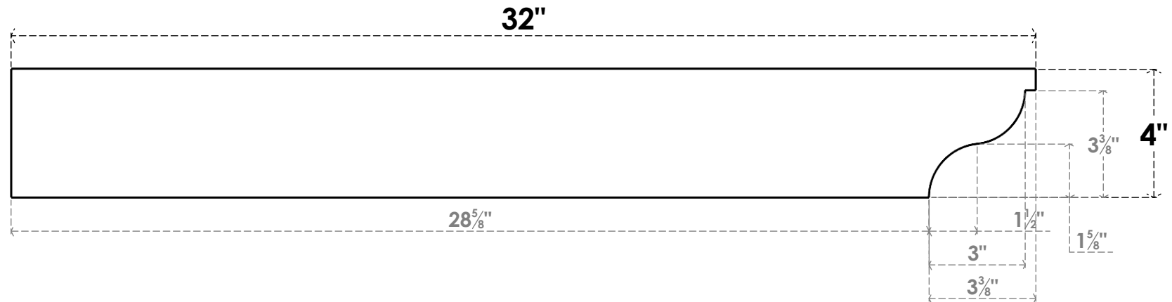
SIDE PROFILE
