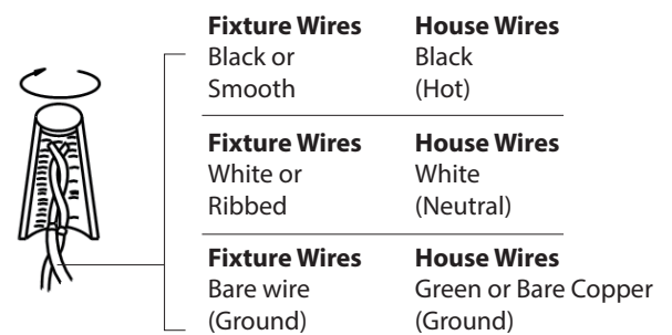
Fig.2 Wiring
