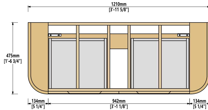
Top view of the cabinet body
