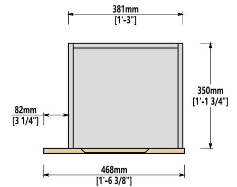
Top view of the right drawer
