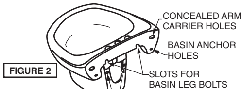
FIGURE 2 SEMI-PEDESTAL/SHROUD* ANCHOR HOLES *SHROUD SOLD SEPARATELY
