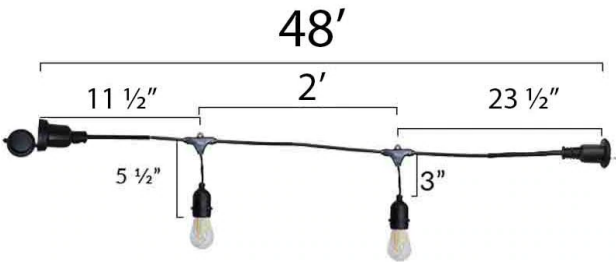
12 & 24 LIGHT STRING DIMENSIONS (available in 24' and 49' lengths)
