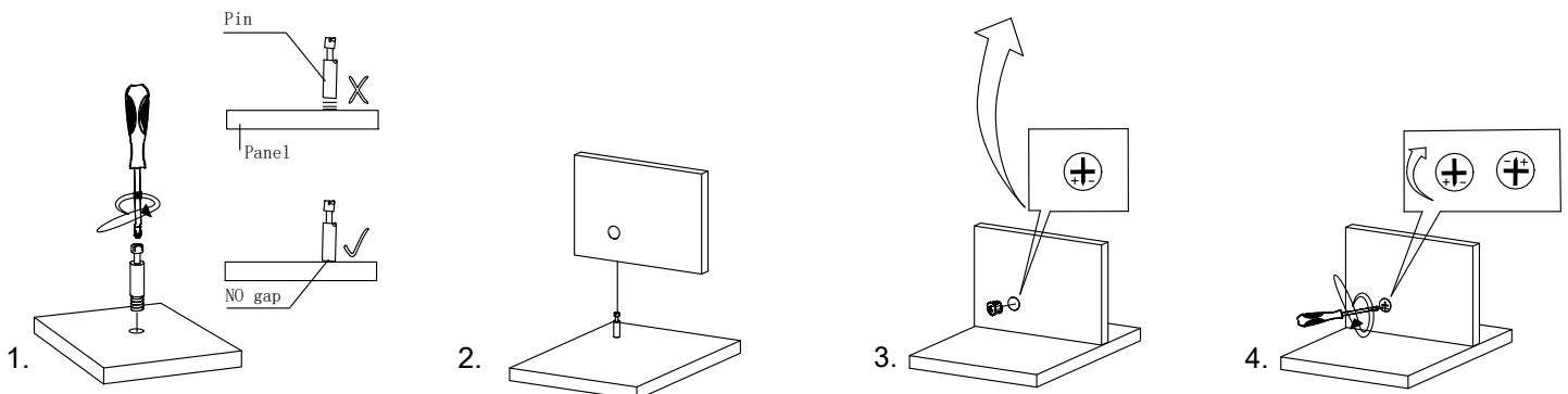
Connecting piece
