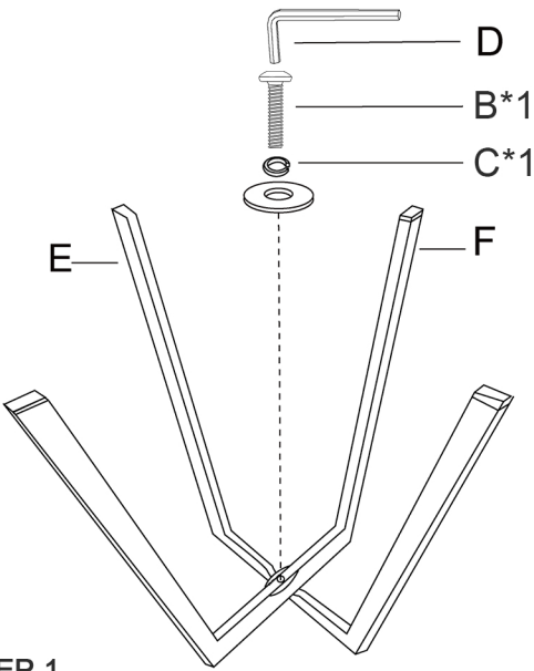
STEP 1. Secure leg (E) and leg (F) with screw (B*1) and washers (C*1).
