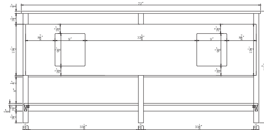
Back view
