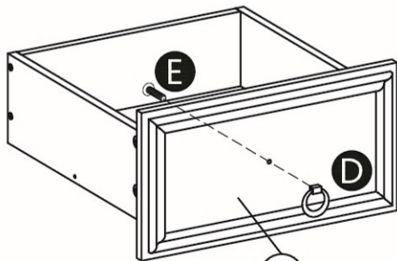
16 Left drawer
