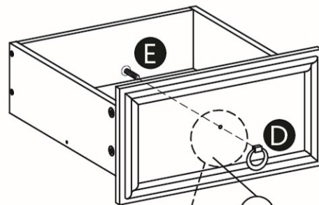
17 Right drawer
