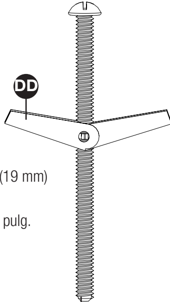
#10 x .75 Pan Head
