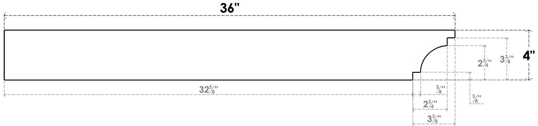
SIDE PROFILE
