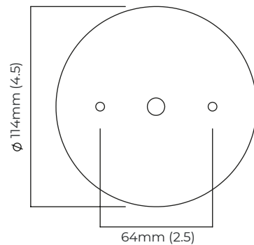
mounting plate dimensions
