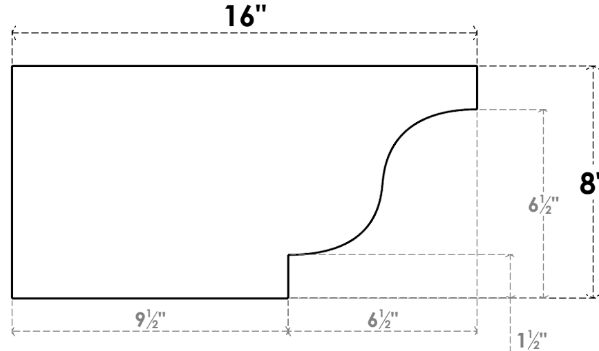
SIDE PROFILE
