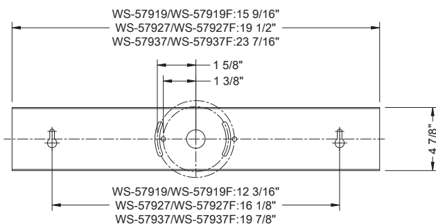
Back Plate Dimensions
