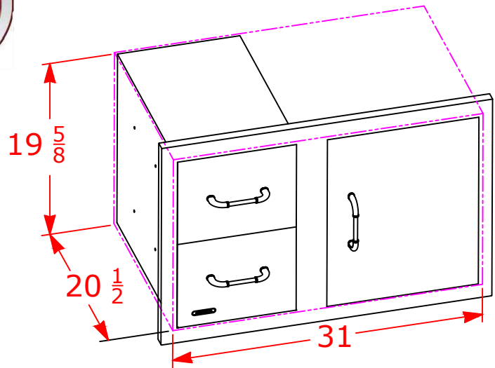
PERSPECTIVE VIEW WITH INSTALLATION CUT OUT DIMENSIONS
