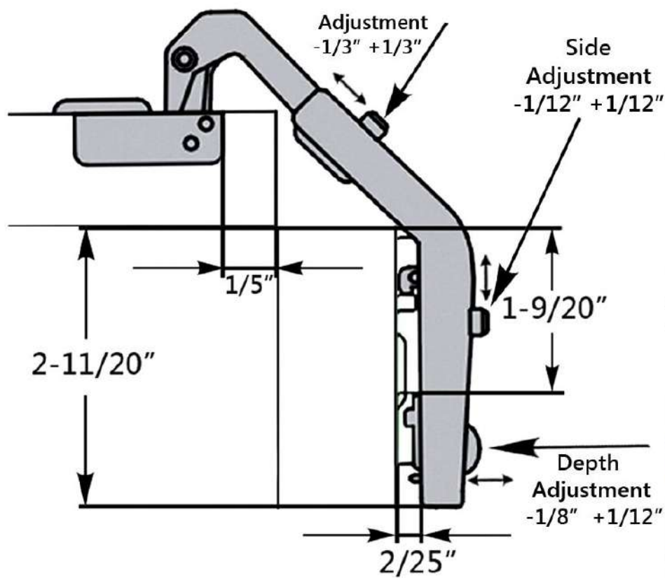
135 Degree Self Closing Full Overlay Hinge
