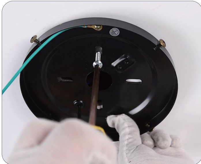
10. Tighten the screws to secure the hanger
