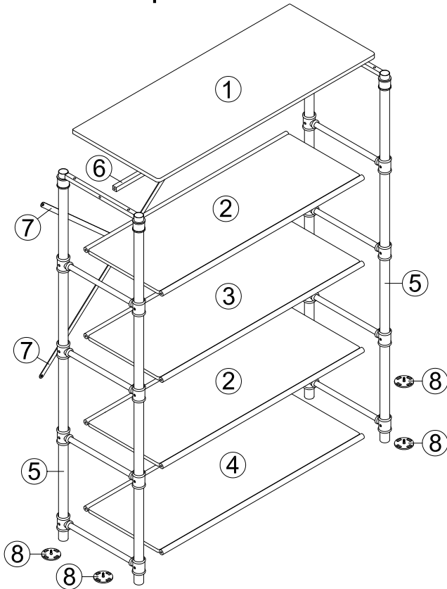
Exploded View
