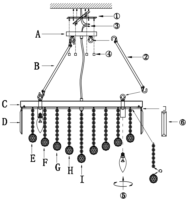
Installation sequence diagram
