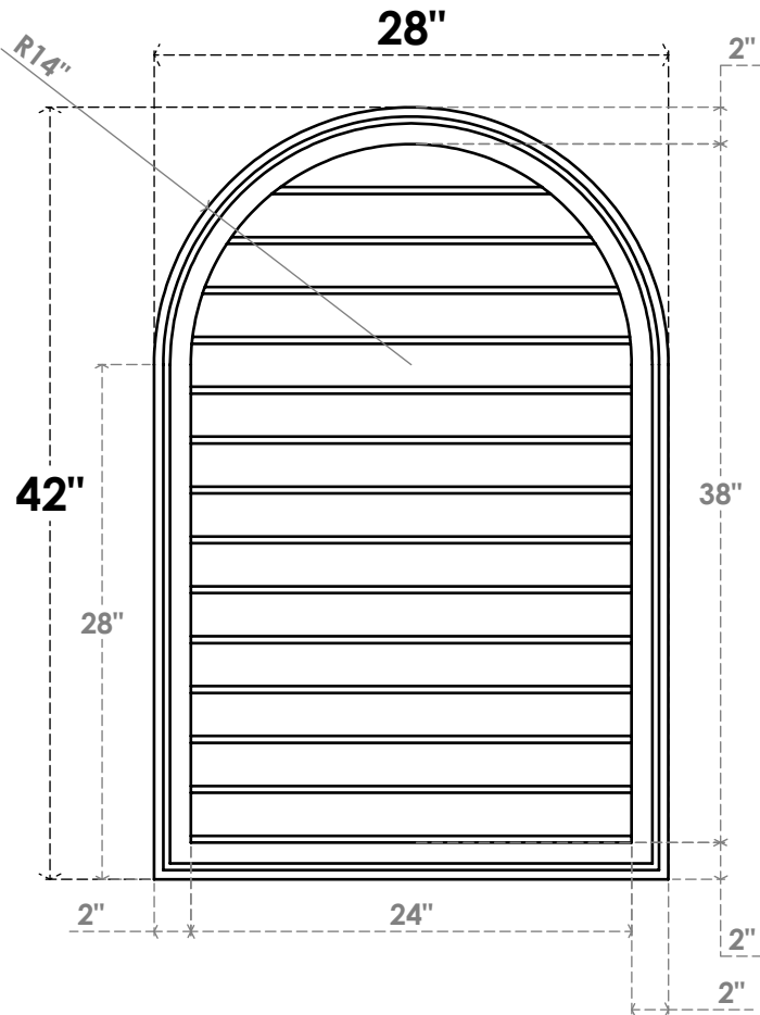
FRONT
