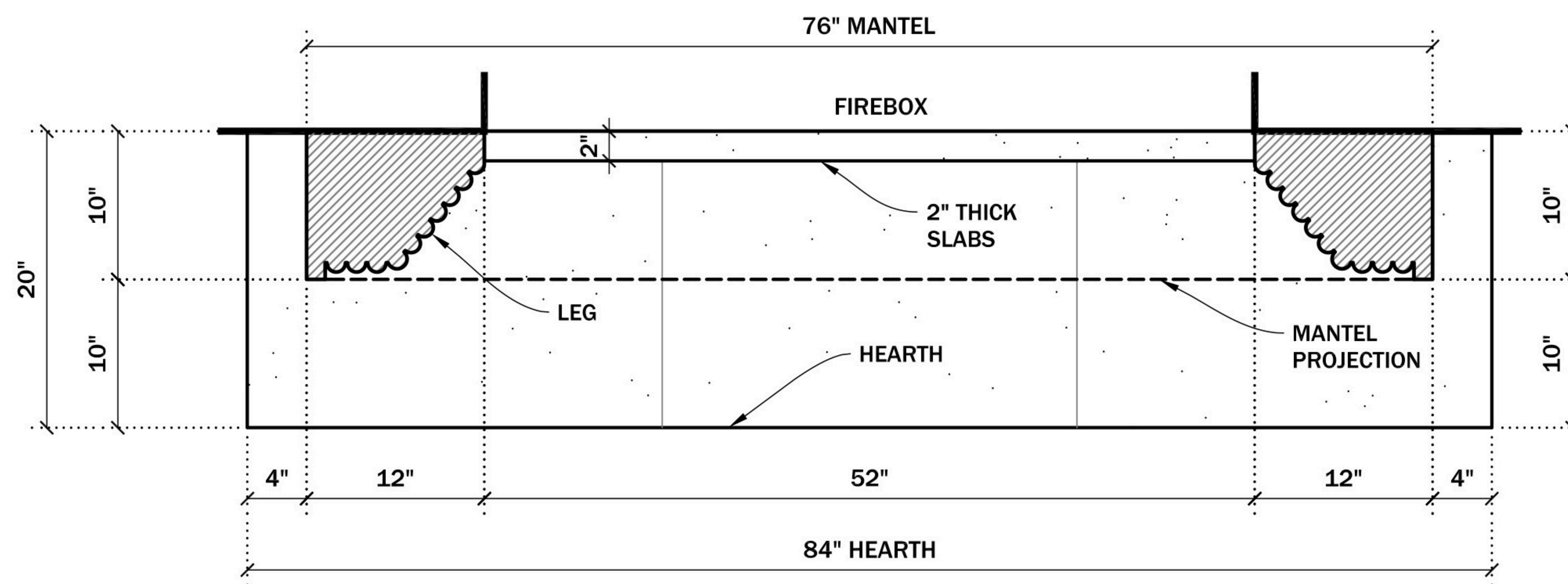
PLAN VIEW
