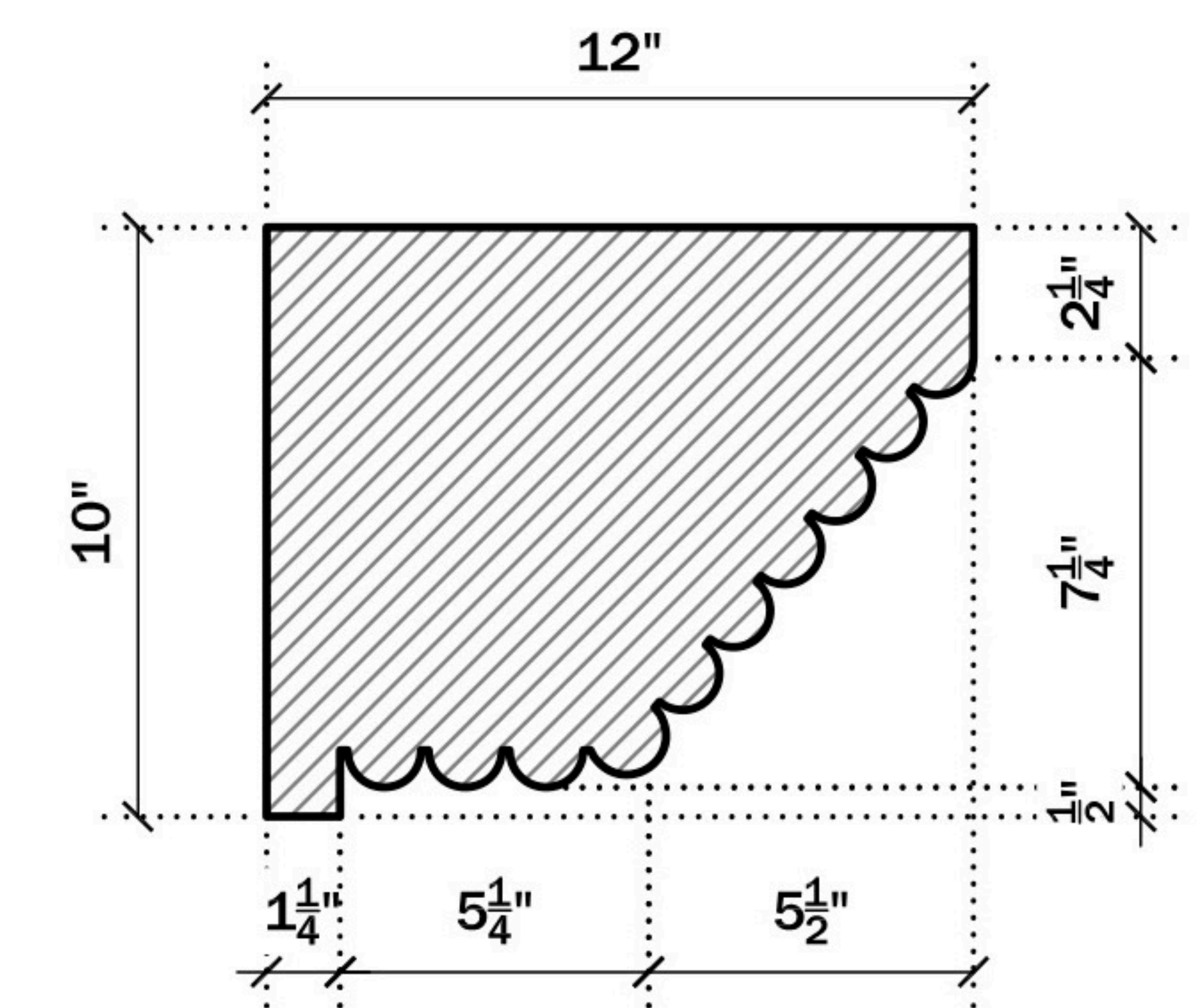
LEGS PROFILE
