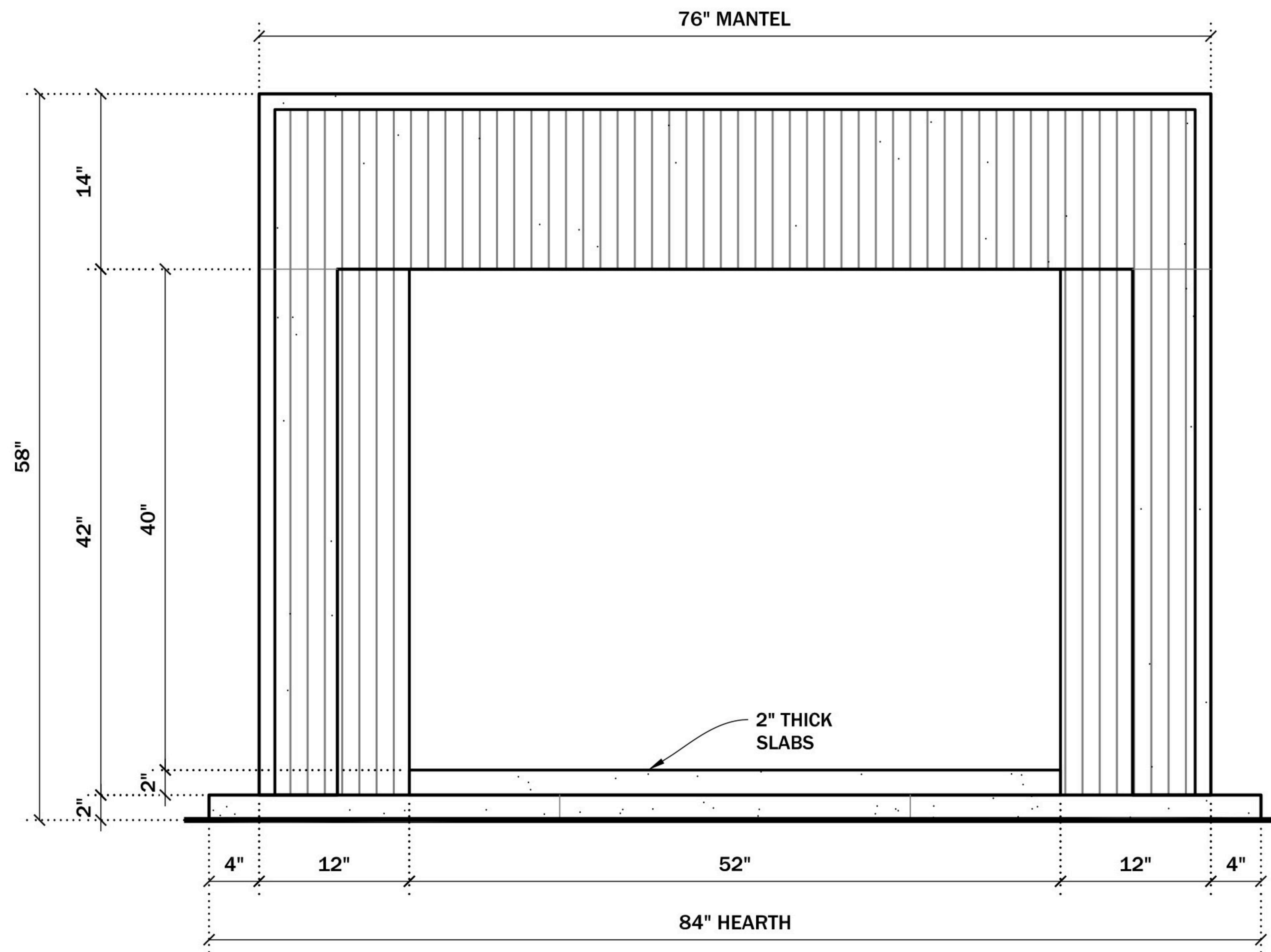
FRONT ELEVATION
