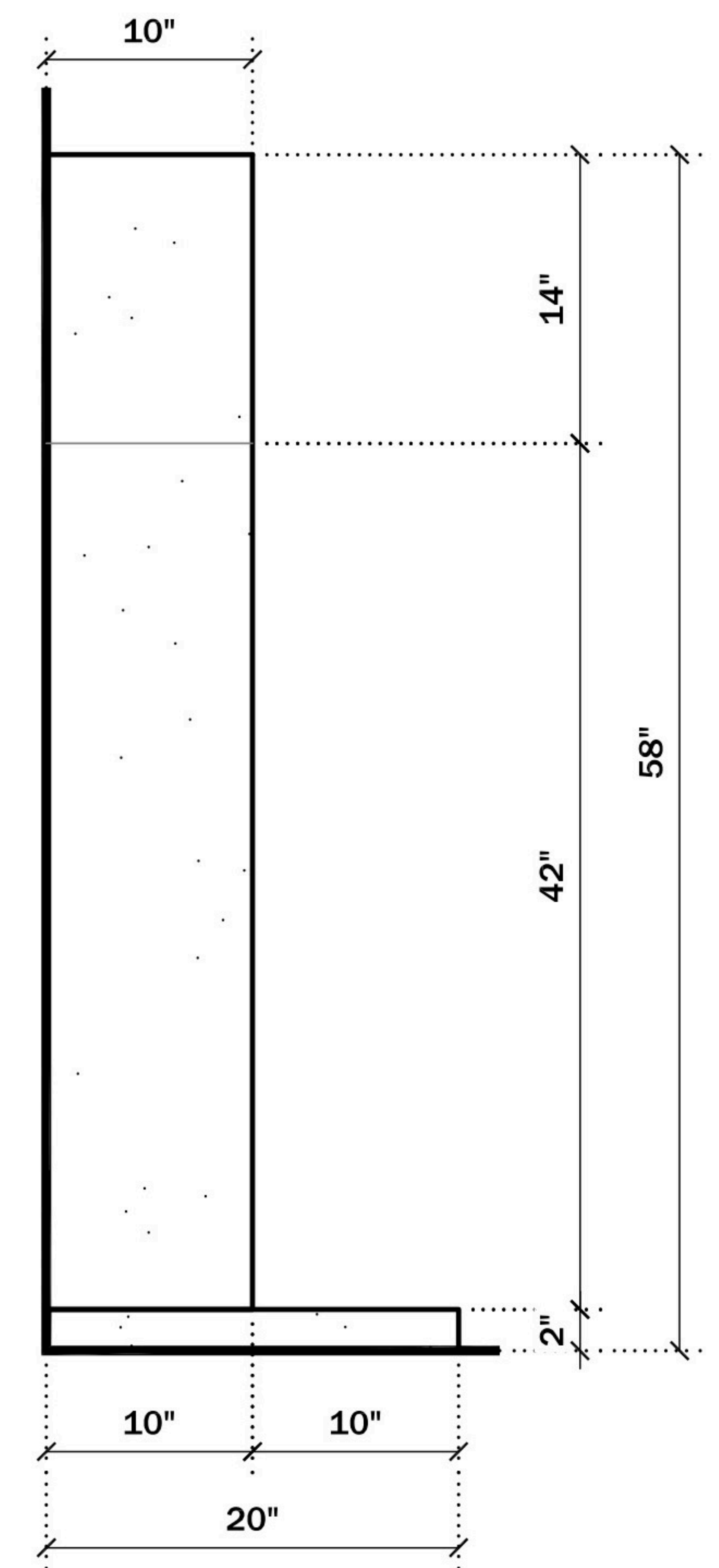
SIDE VIEW
