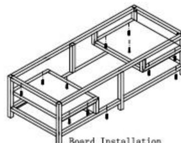
Board Installation
