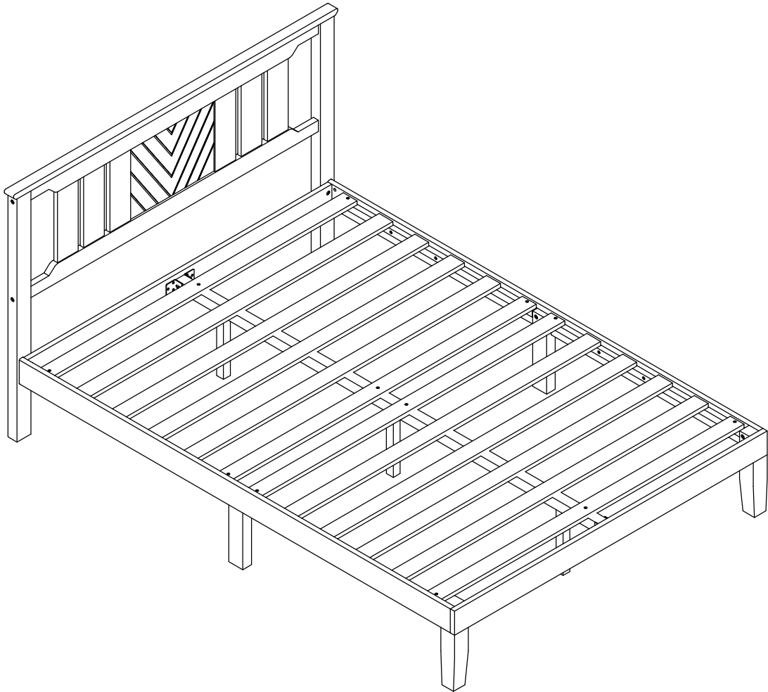
Wood Platform Bed Frame with solid wood headboard Full
