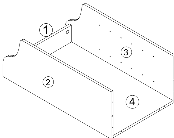
Completed Assembly
