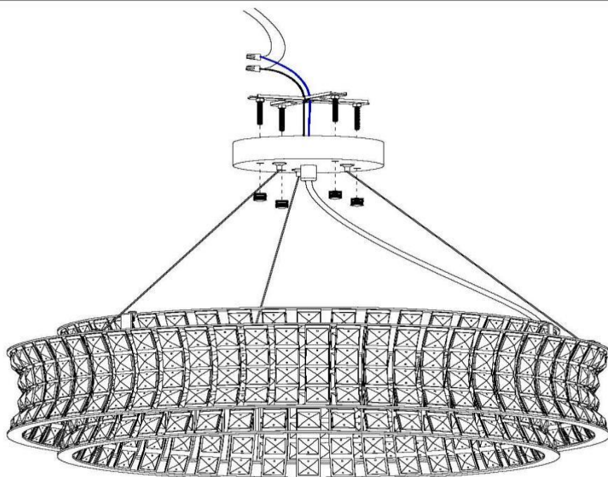
EXPLODED VIEW
