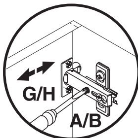
LATERAL ADJUSTMENT
