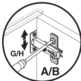
HEIGHT ADJUSTMENT
