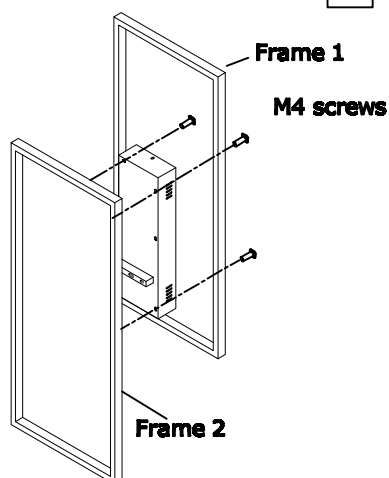
assemble frame 2
