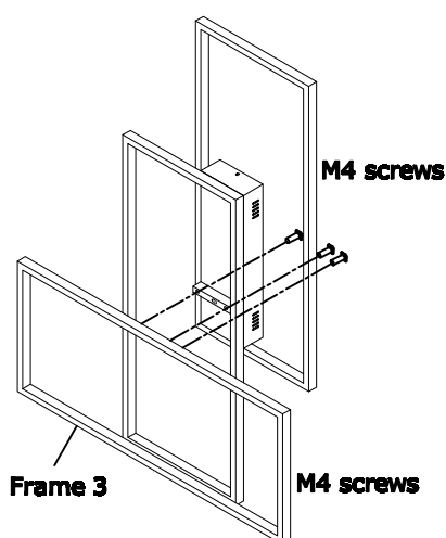
assemble frame 3
