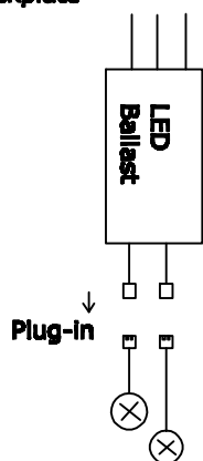
plugs connection inside backplate
