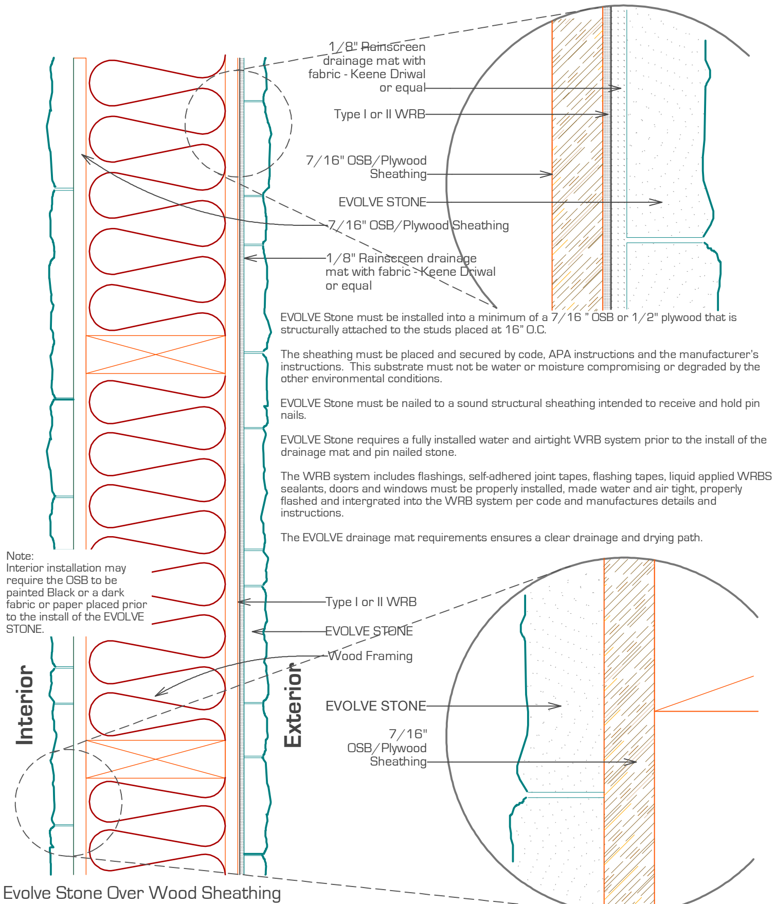
EVOLVE STONE TYPICAL WALL TYPES - DETAIL #9
