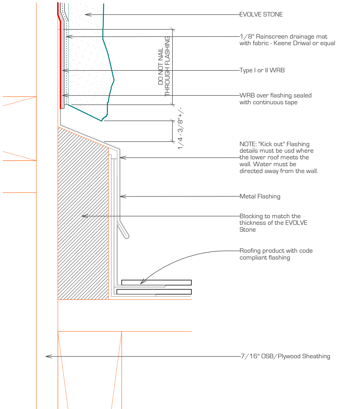
DETAIL #7
