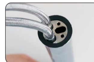
Put O-ring to the position as shown
