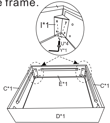
Seat f rame 1
