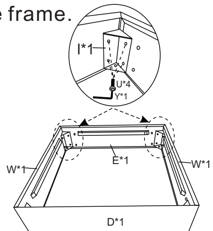
Seat f rame 3
