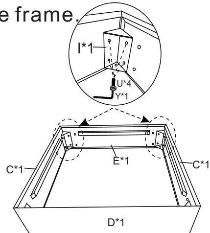
Seat f rame 2
