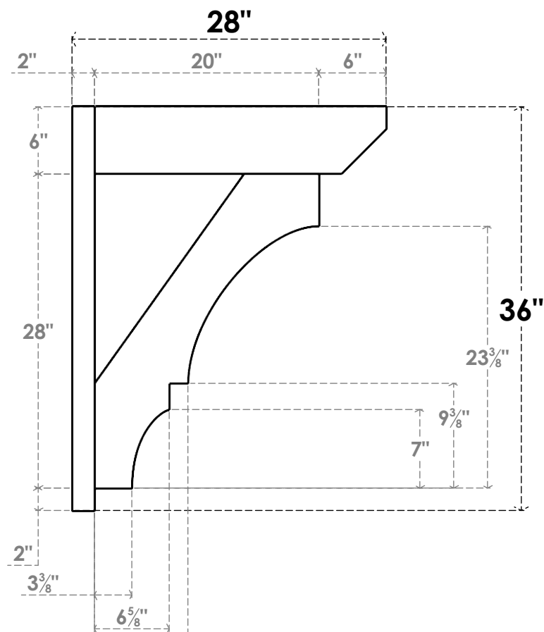
SIDE PROFILE
