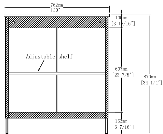
Back View
