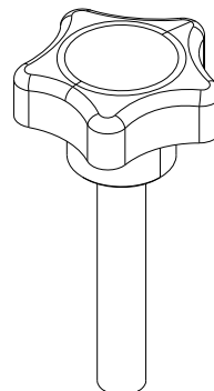
Handle Bolt: M8x40
