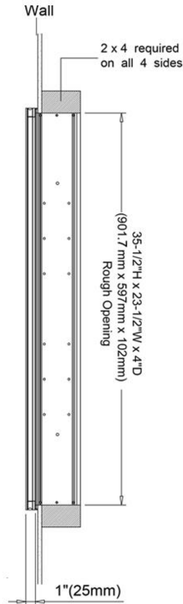
Recessed Mount
