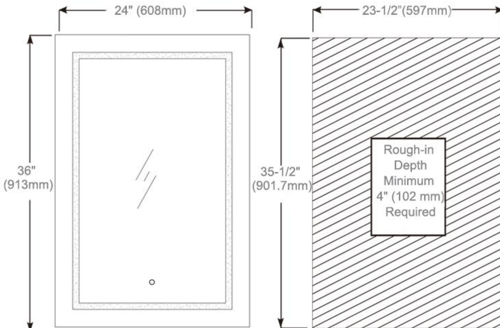
Cabinet Dimensions
