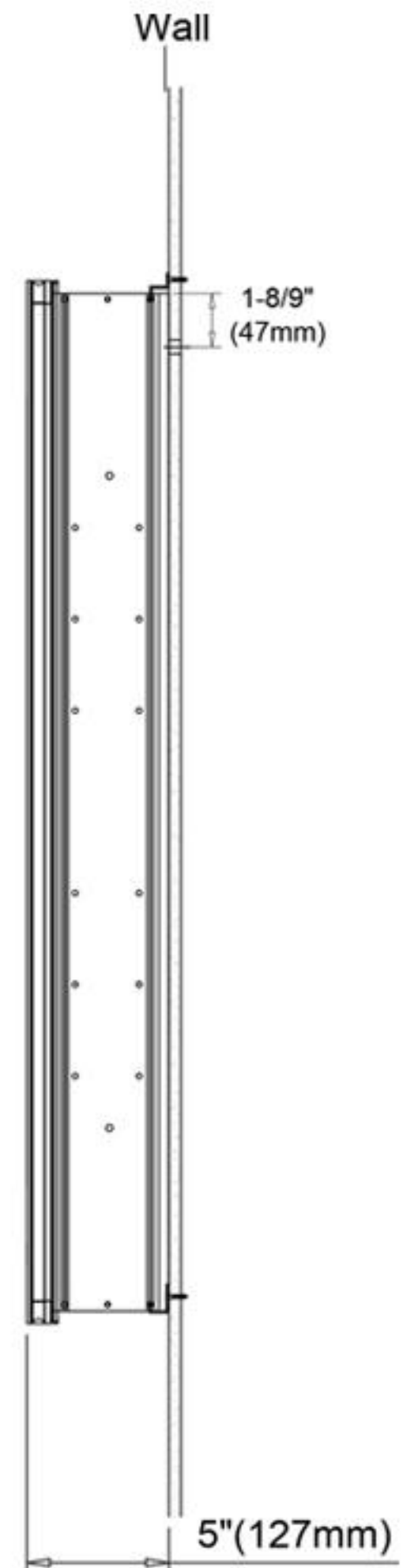
Surface Mount
