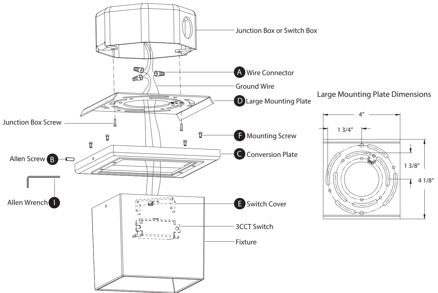
FIG. 5 MOUNT ON THE JUNCTION BOX OR SWITCH BOX
