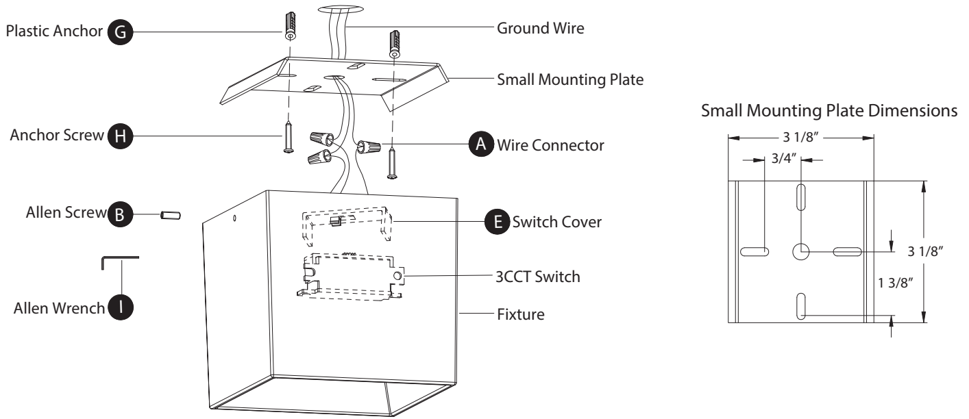
FIG. 1 MOUNT WITHOUT CONVERSION PLATE
