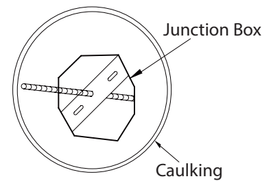
Fig. 4 Sealing
