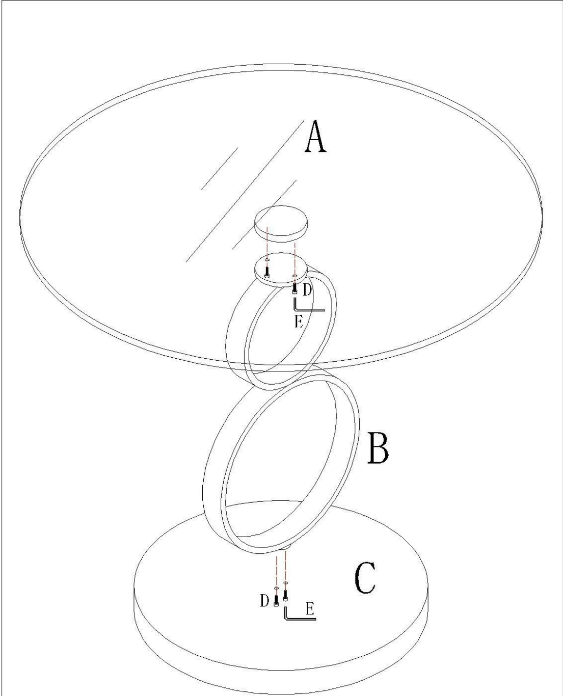
INSTALLATION DIAGRAM
