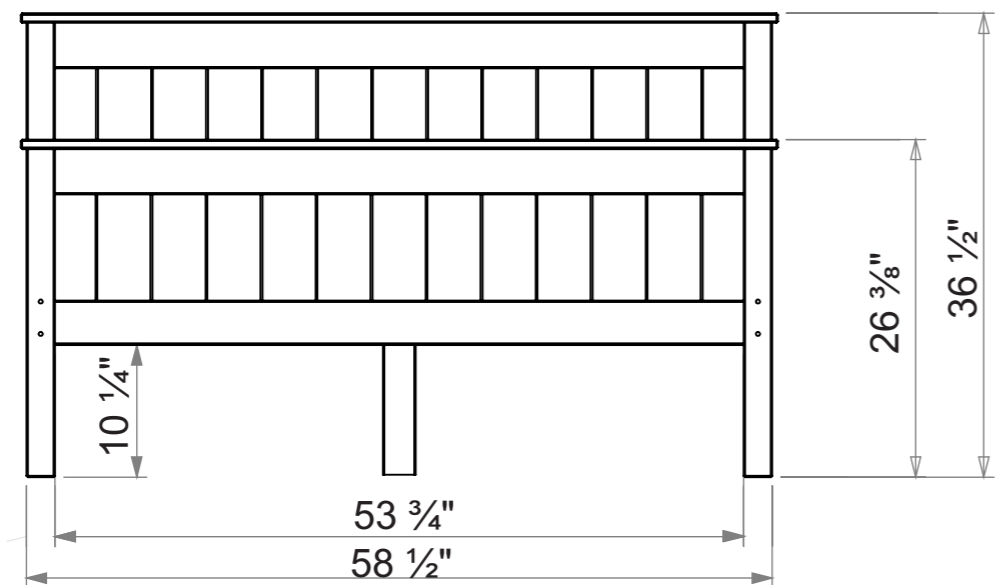
Frontal View
