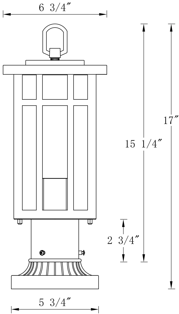
FRONT VIEW
